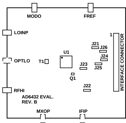
Figure 36. Evaluation Board Layout (Top View)
