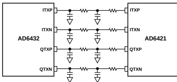
Figure 34. GSM Phase II Transmit Interface
