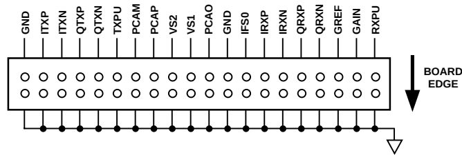
Figure 37. Evaluation Board Interface Connector
