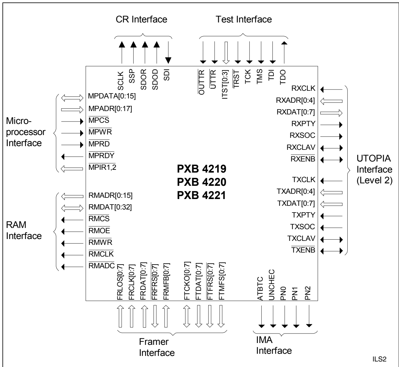
Figure 1 Logic Symbol
