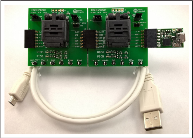
Figure 1. DS28E36EV with USB Cable
