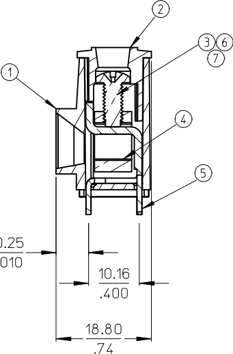
SECTION Z-Z
