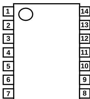
NJM2166E/V
