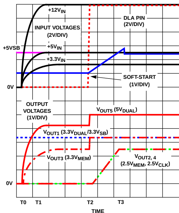
FIGURE 8. SOFT-START INTERVAL IN ACTIVE STATE (2.5V/3.3V MEM OUTPUT SHOWN IN 2.5V SETTING)
