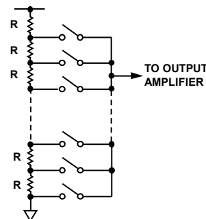
Figure 30. Resistor String
