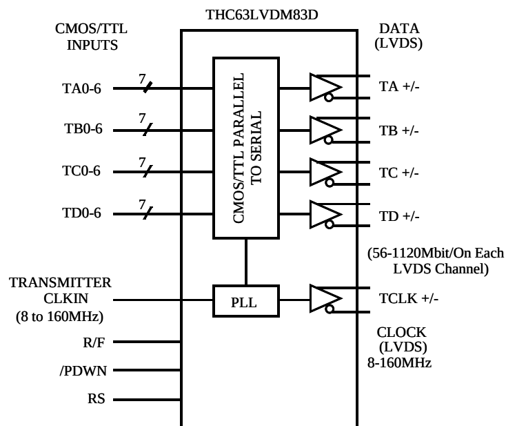
Figure 1. Block Diagram
