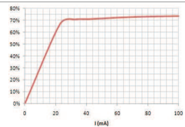
Figure 4. BUCK2 Efficiency
