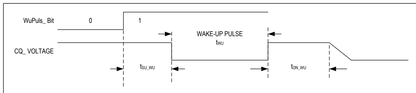
Figure 9. Wake-Up Timing
