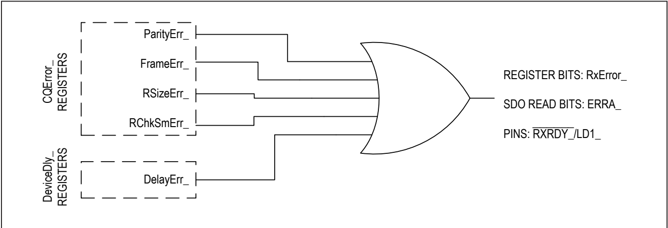
Figure 18. RxError_ Triggers
