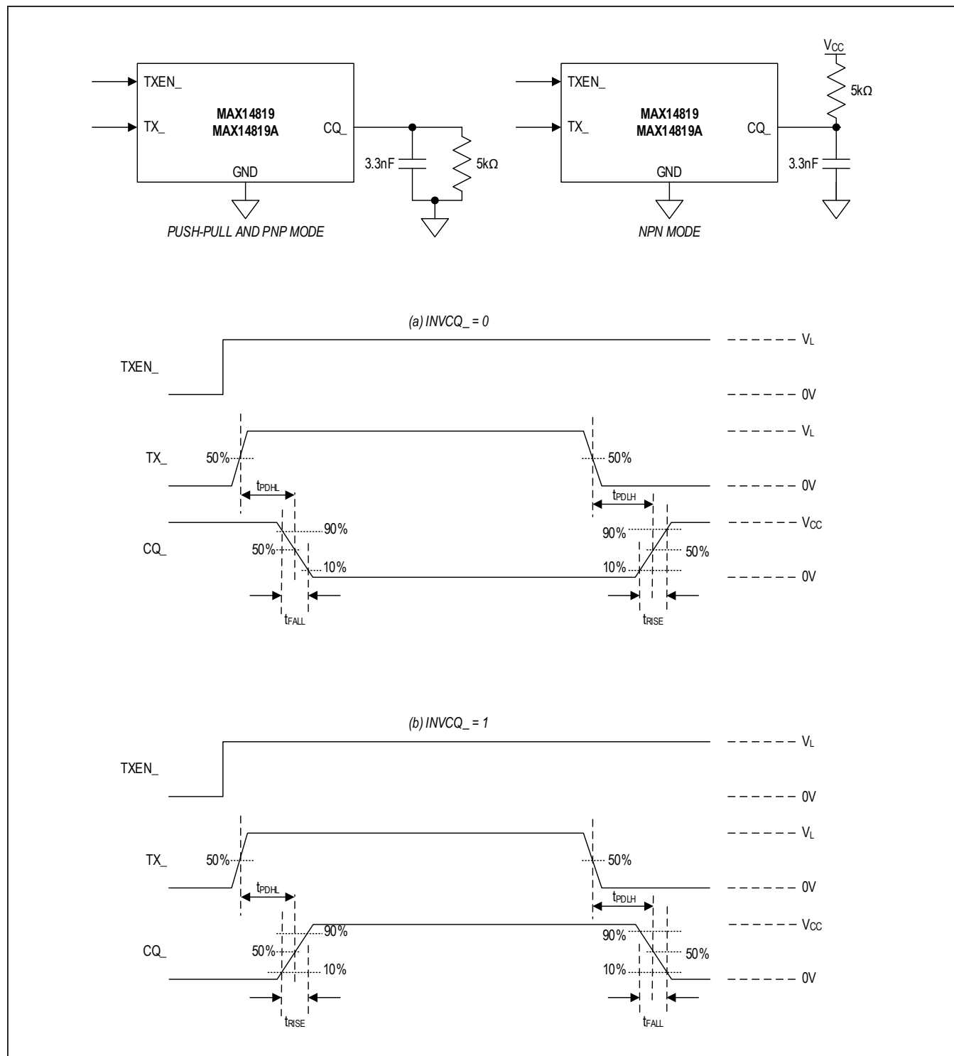
Figure 1. C/Q Driver Propagation Delays and Rise/Fall Times
