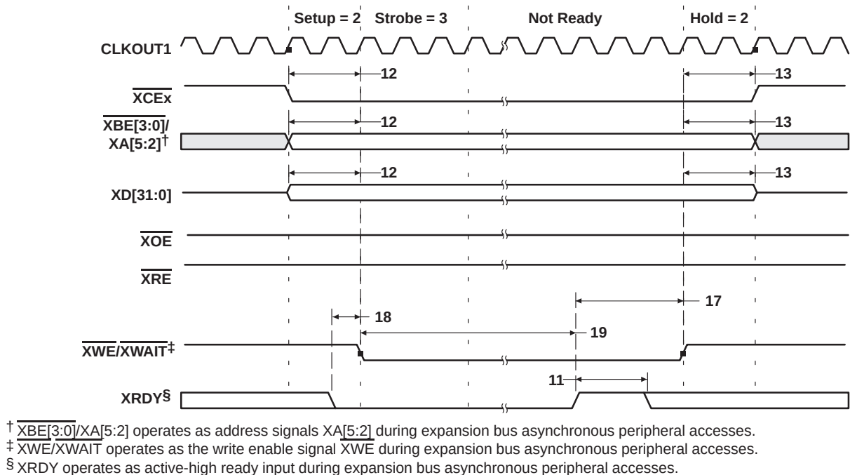
Figure 34. Expansion Bus Asynchronous Peripheral Write Timing (XRDY Used)
