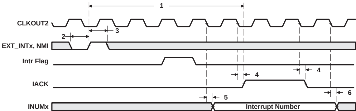
Figure 27. Interrupt Timing
