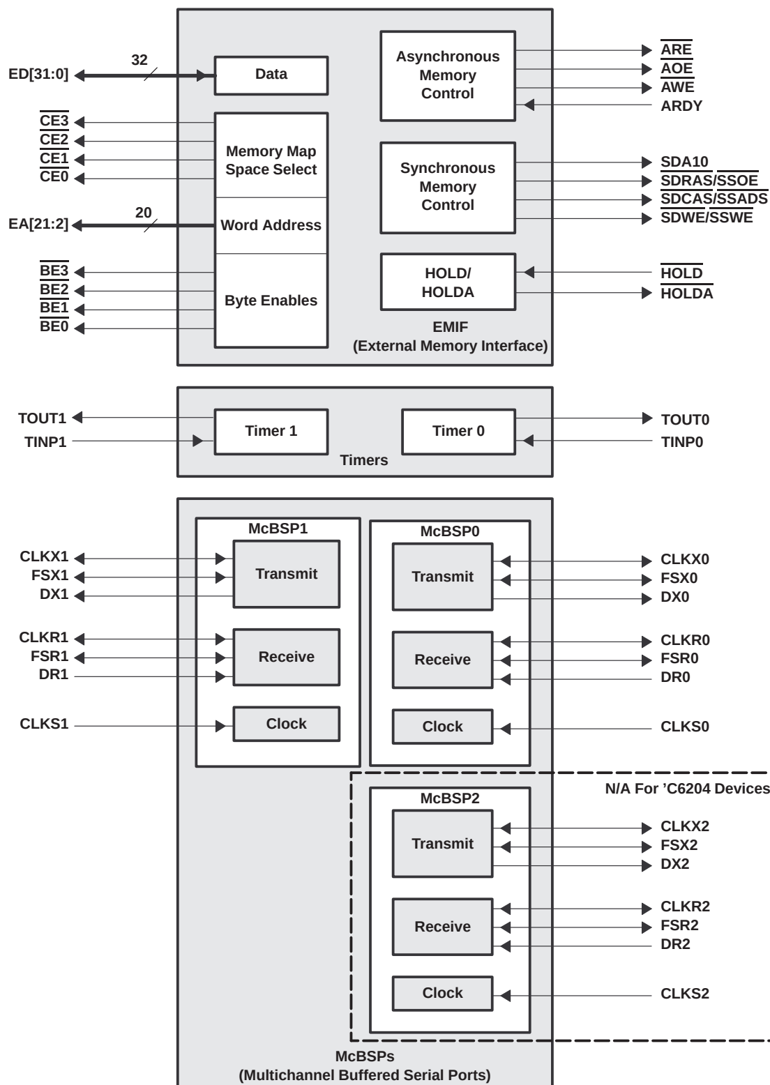
Figure 3. Peripheral Signals
