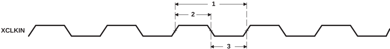
Figure 10. XCLKIN Timings
