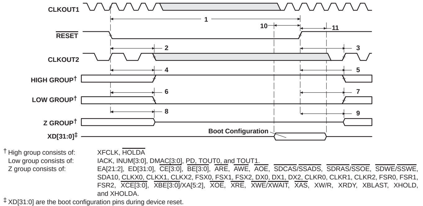
Figure 26. Reset Timing
