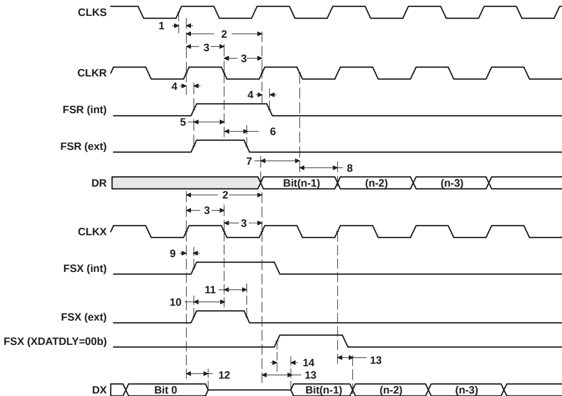
Figure 44. McBSP Timings
