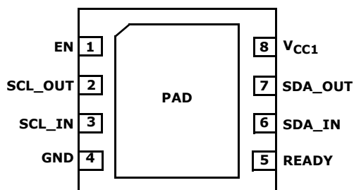
ISL33001 (8 LD TDFN) TOP VIEW
