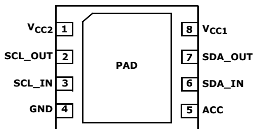
ISL33003 (8 LD TDFN) TOP VIEW
