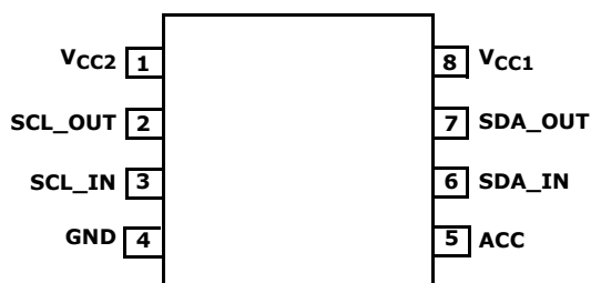
ISL33003 (8 LD MSOP) TOP VIEW
