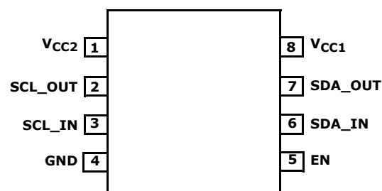
ISL33003 (8 LD MSOP) TOP VIEW
