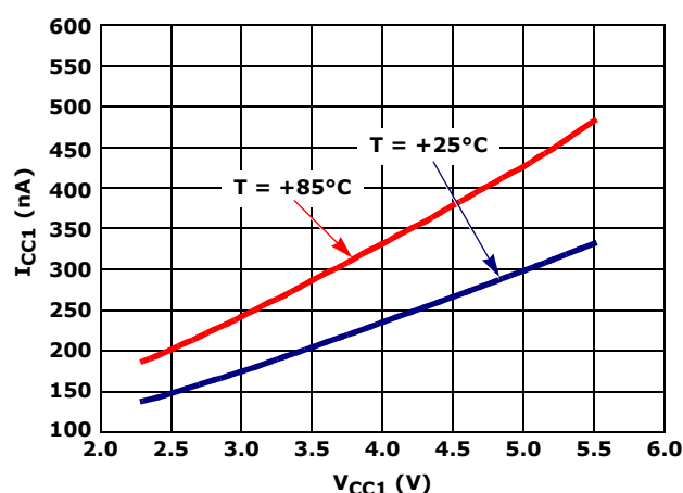
FIGURE 10. I_{CC1} DISABLED CURRENT vs V_{CC1} (ISL33001)
