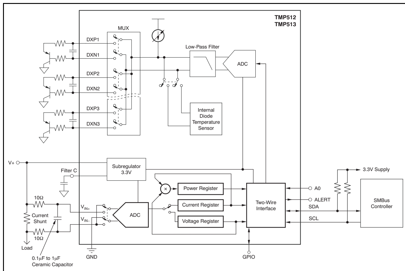
Figure 28. TMP512/13 with Input Filtering
