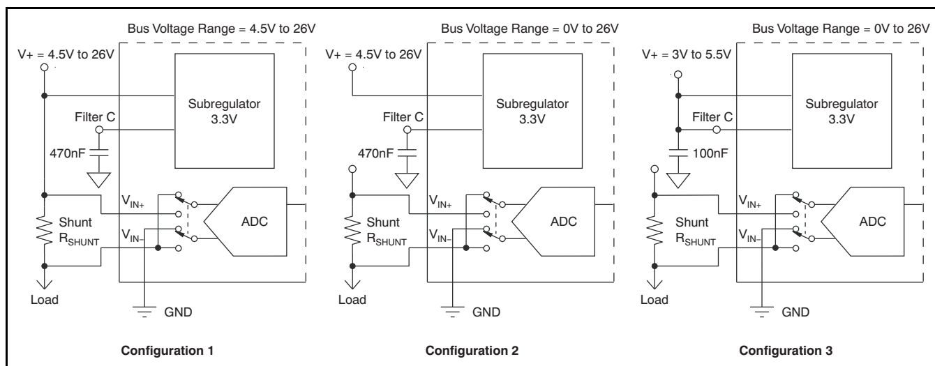
Figure 20. Typical Subregulator Configurations
