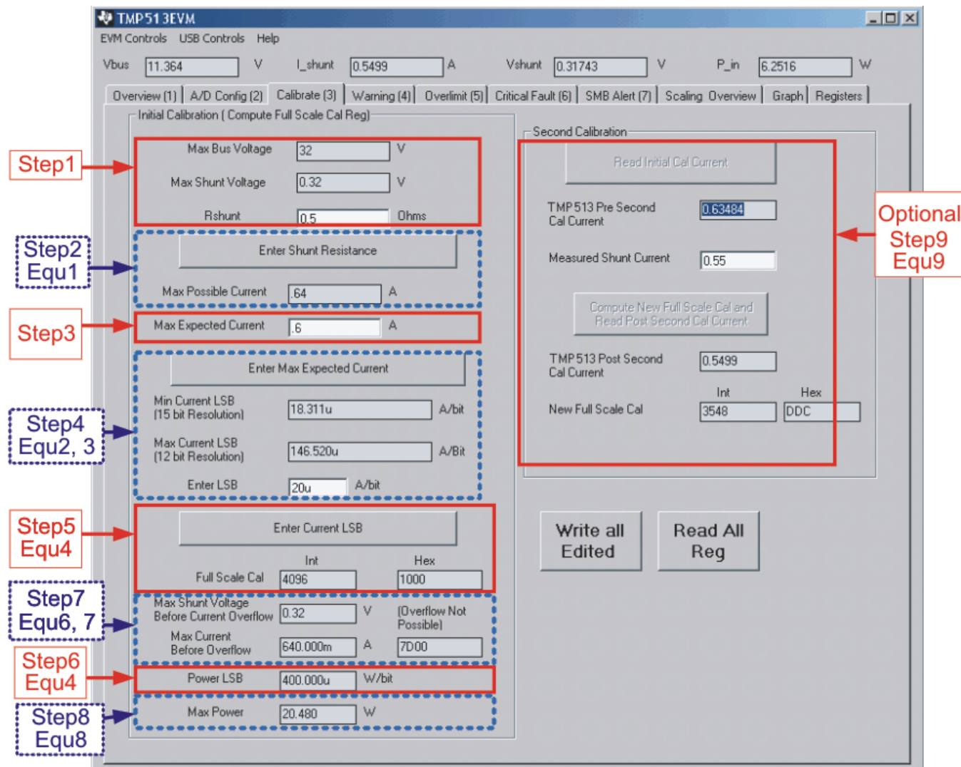
Figure 30. TMP512/513EVM Calibration Software Automatically Computes Calibration Steps 1-9
