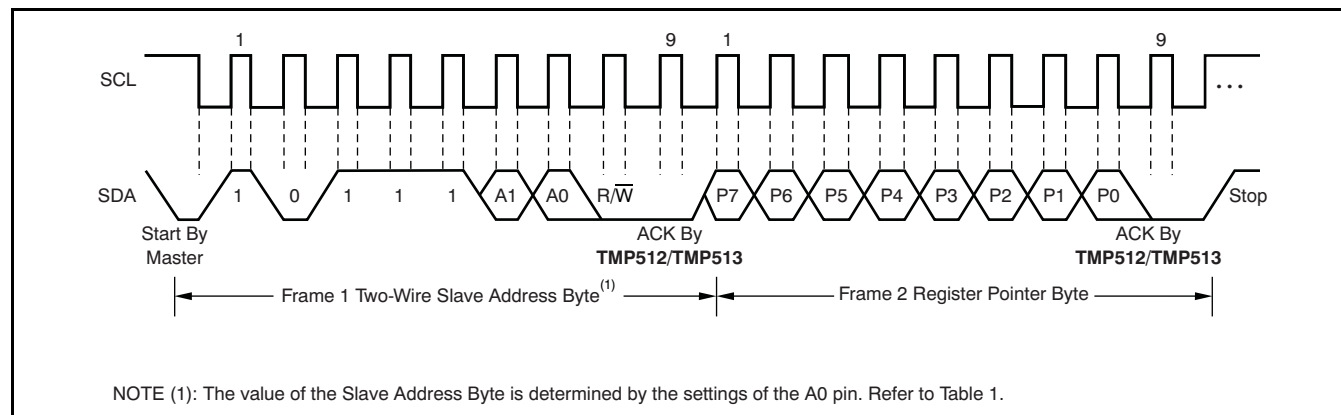
Figure 25. Typical Register Pointer Set
