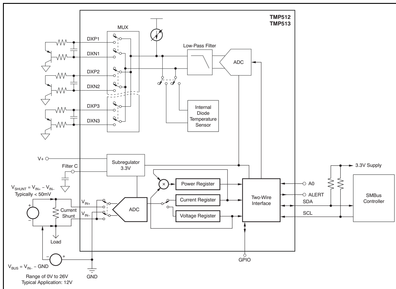
Figure 27. TMP512/13 Configured for Shunt and Bus Voltage Measurement
