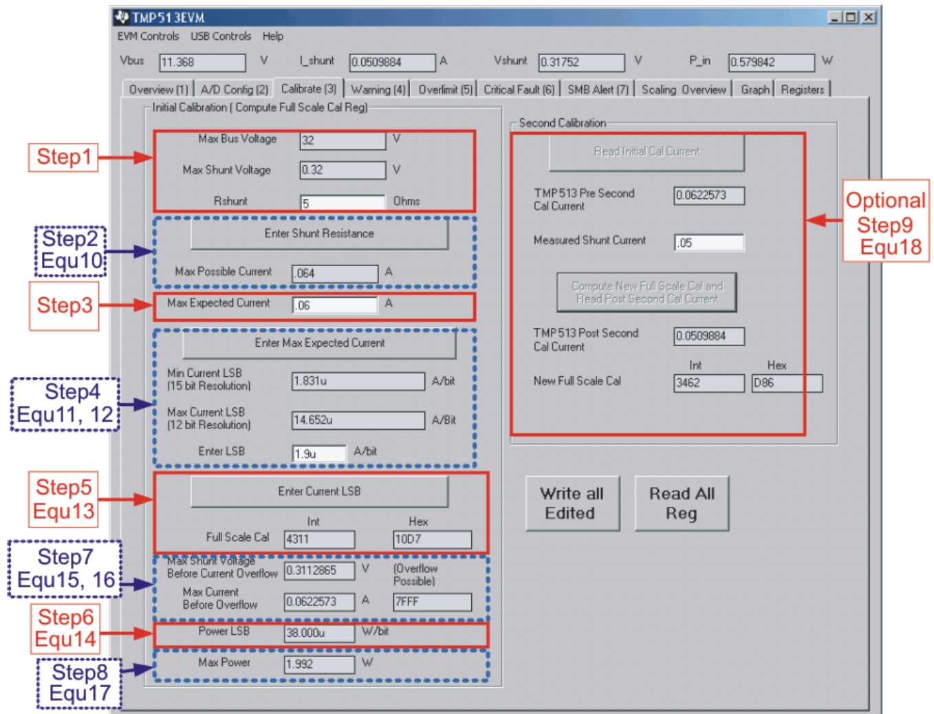
Figure 31. TMP512/513EVM Calibration Software Automatically Computes Calibration Steps 1-9
