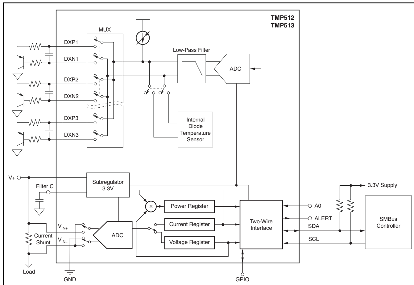
Figure 21. Typical Application Circuit
