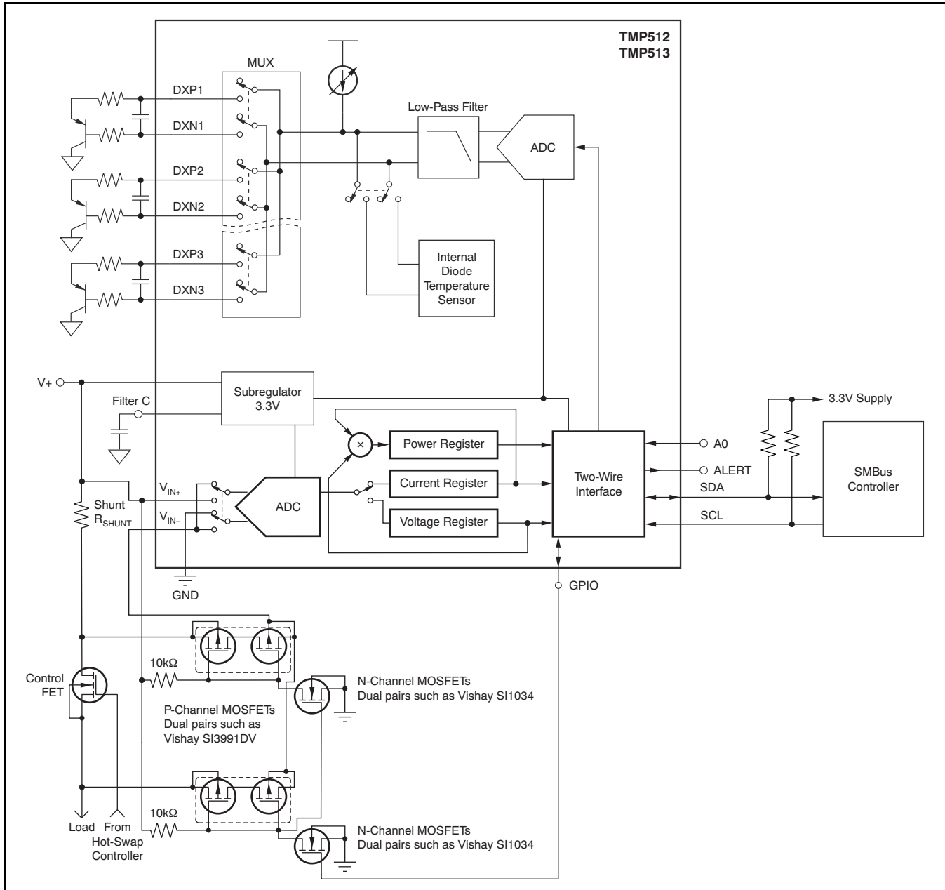
Figure 29. External Circuitry for Additional V_{BUS} Input
