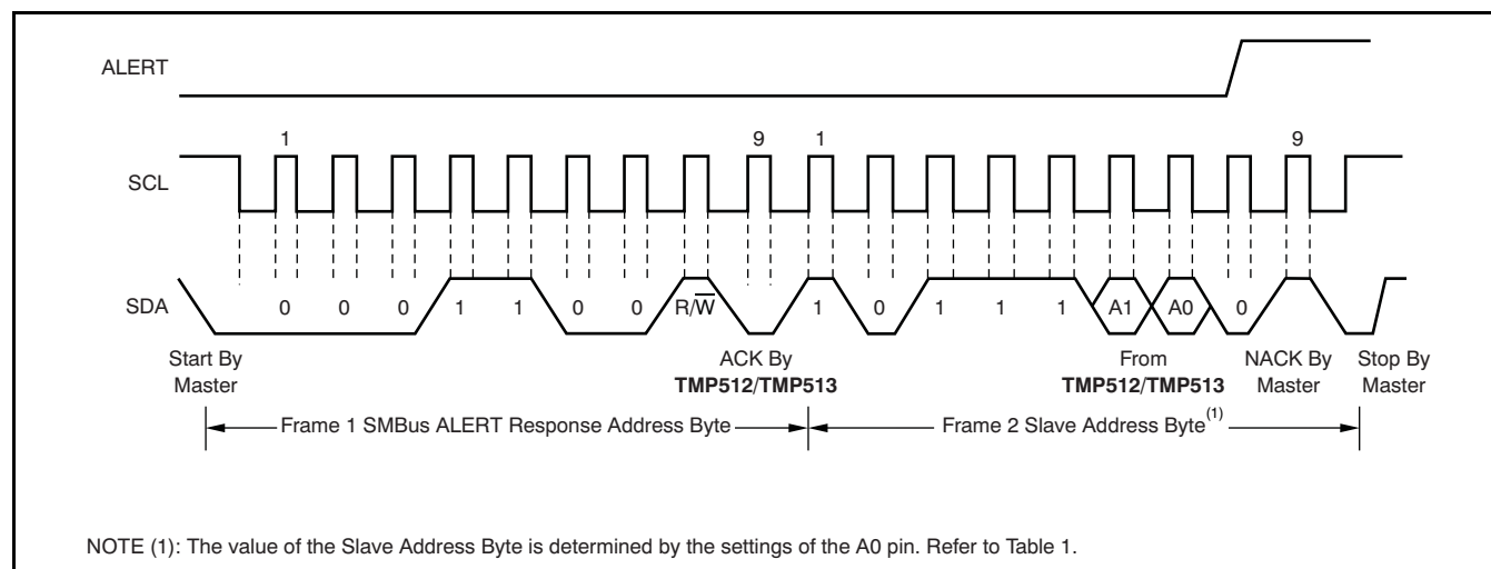
Figure 24. Timing Diagram for SMBus ALERT
