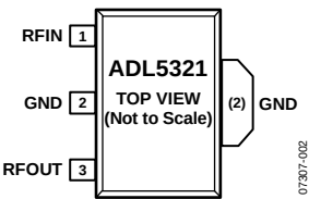
Figure 3. Pin Configuration
