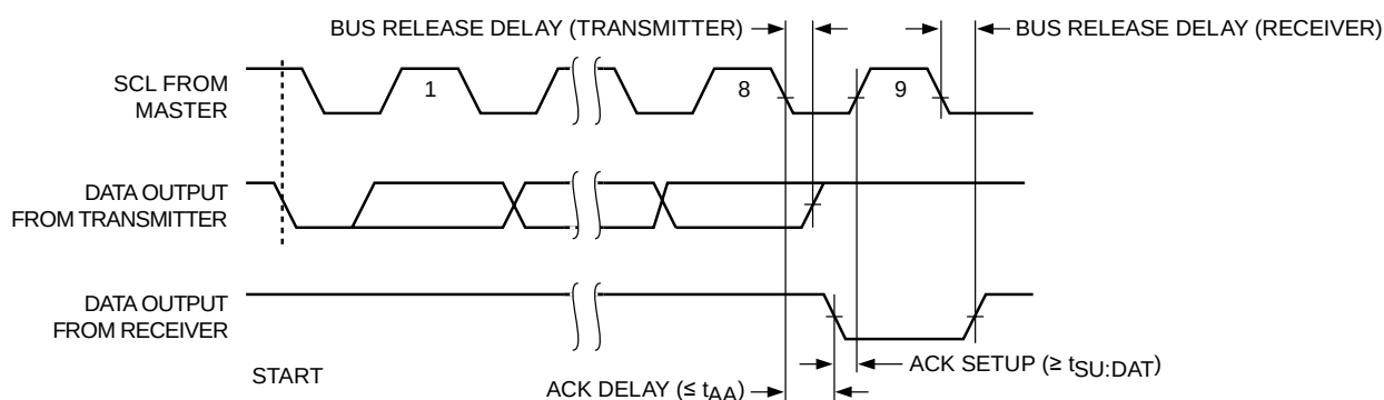
Figure 6. Bus Timing
