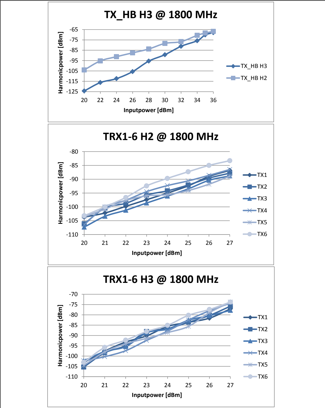
Figure 35 Measurements of Harmonic power over Carrier power of High-Band inputs to HB Antenna
