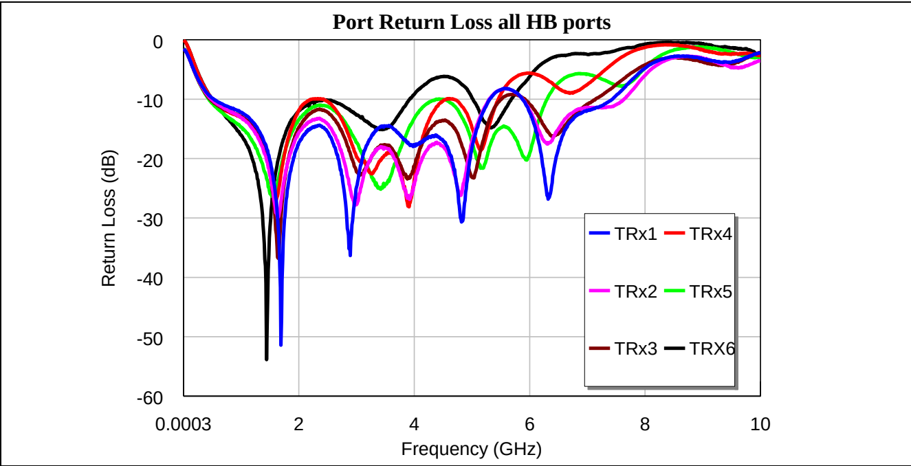
Figure 24 Return Loss from HB TRX RF ports to HB Antenna
