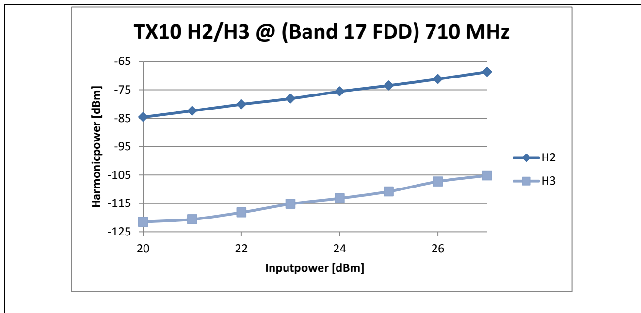
Figure 34 Harmonic power measurements of high linear LB input TRX10 over the Band 17 carrier
