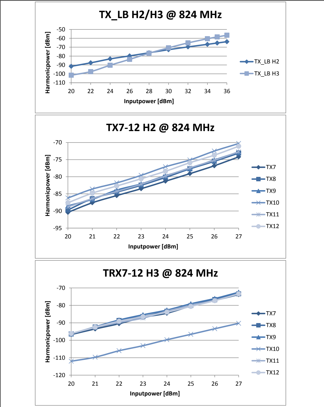
Figure 33 Measurements of Harmonic power over Carrier power of Low-Band inputs to LB Antenna
