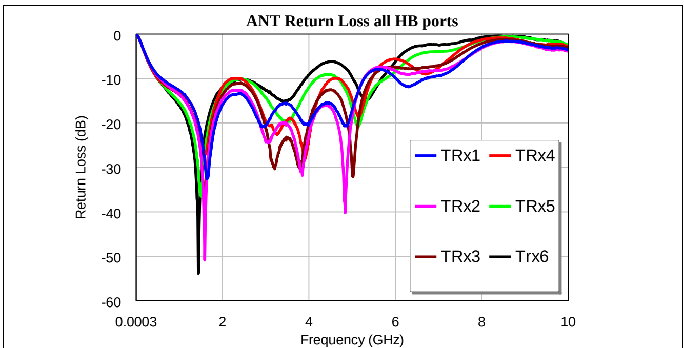
Figure 23 Return Loss from HB Antenna to the respective TRX HB RF port
