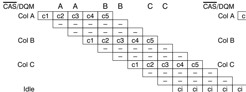
Figure 57. DRAM Cycle Column Pipelines
