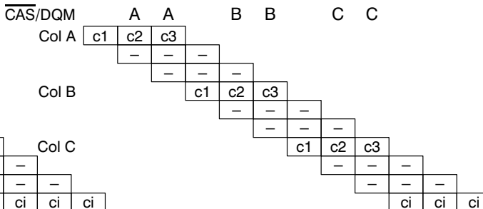
Figure 57. DRAM Cycle Column Pipelines
