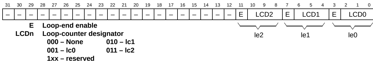
Figure 29. lctl Register
