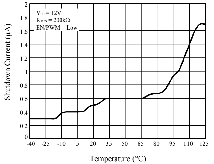
Figure 5 I_{SD} vs. T_J
