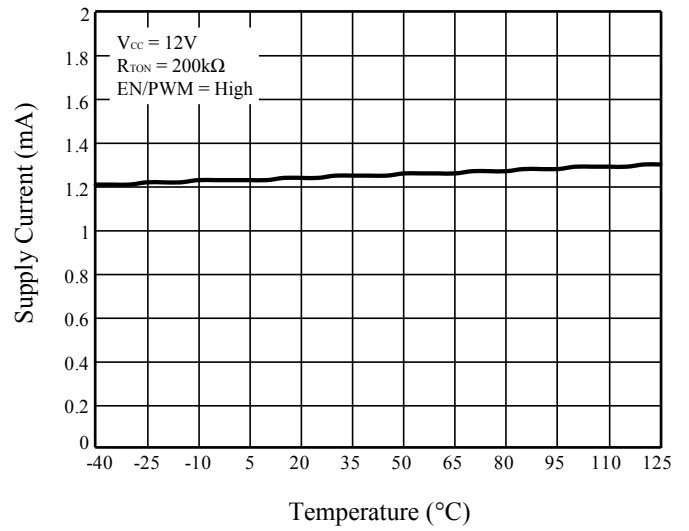
Figure 3 I_{CC} vs. T_J
