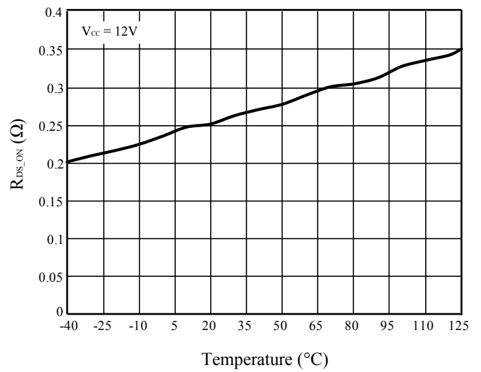
Figure 7 R_{DS\_ON} vs. T_J
