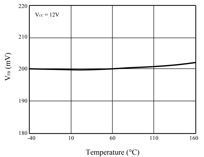
Figure 13 V_{FB} vs. T_J
