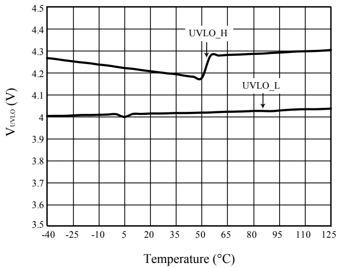
Figure 12 V_{UVLO} vs. T_J
