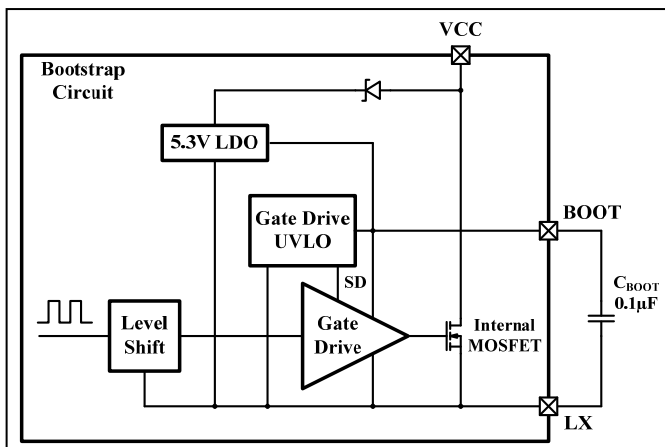
Figure 26 Bootstrap Circuit
