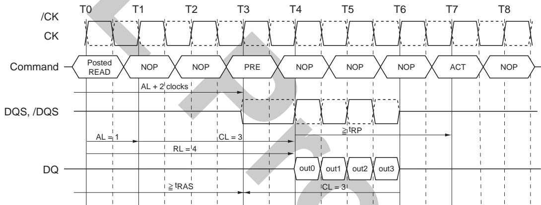
Burst Read Operation Followed by Precharge (RL = 4 (AL=1, CL=3))
