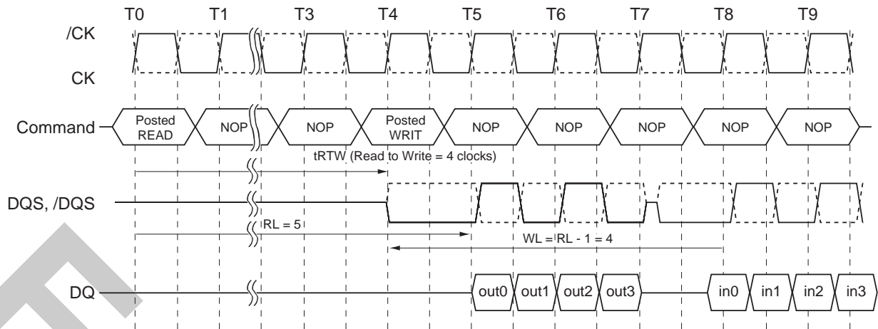
Burst Read followed by Burst Write (RL = 5, WL = RL-1 = 4)
