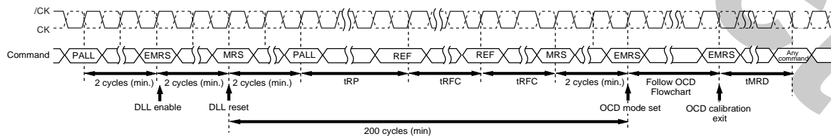
Power up and Initialization Sequence
