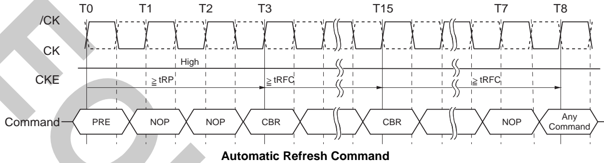
Automatic Refresh Command
