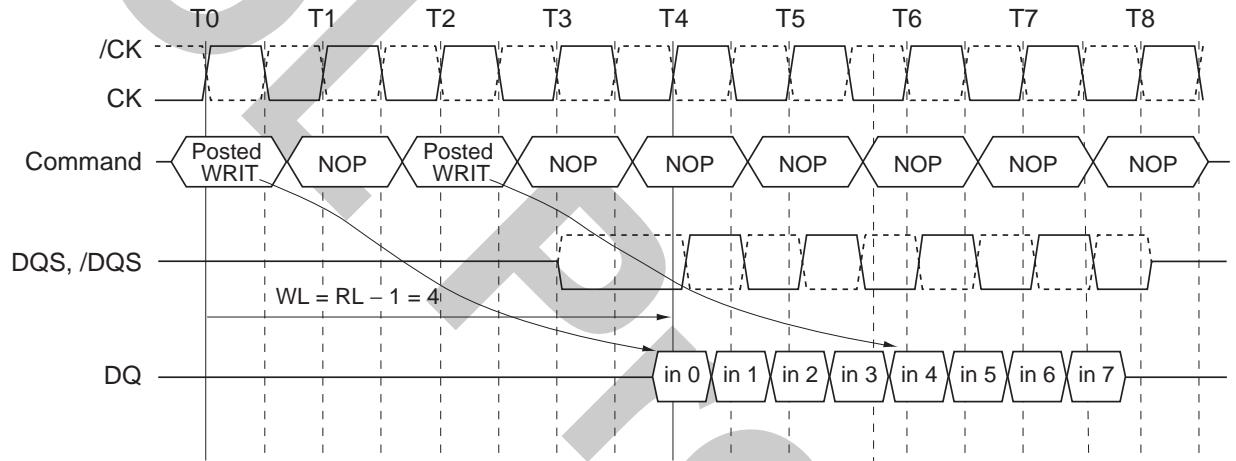
Seamless Burst Write Operation (RL = 5, WL = 4)
