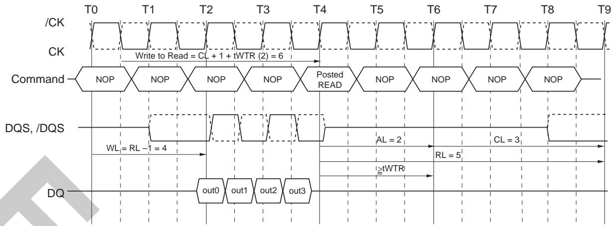
Burst Write followed by Burst Read (RL = 5 (AL=2, CL=3), WL = 4, tWTR = 2)
