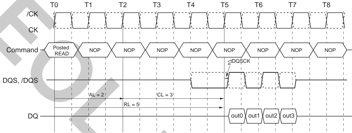
Burst Read Operation (RL = 5 (AL = 2, CL = 3))
