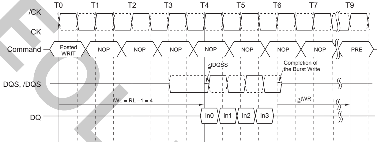
Burst Write Operation (RL = 5, WL = 4, tWR = 3 (AL=2, CL=3))
