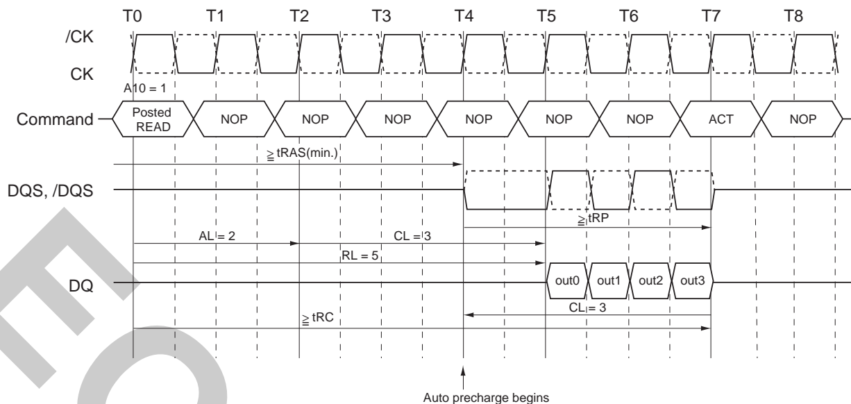
Burst Read with Auto Precharge Followed by an Activation to the Same Bank (tRP limit) RL = 5 (AL = 2, CL = 3, internal tRCD = 3)
