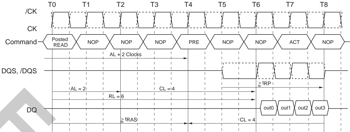
Burst Read Operation Followed by Precharge (RL = 6 (AL=2, CL=4))
