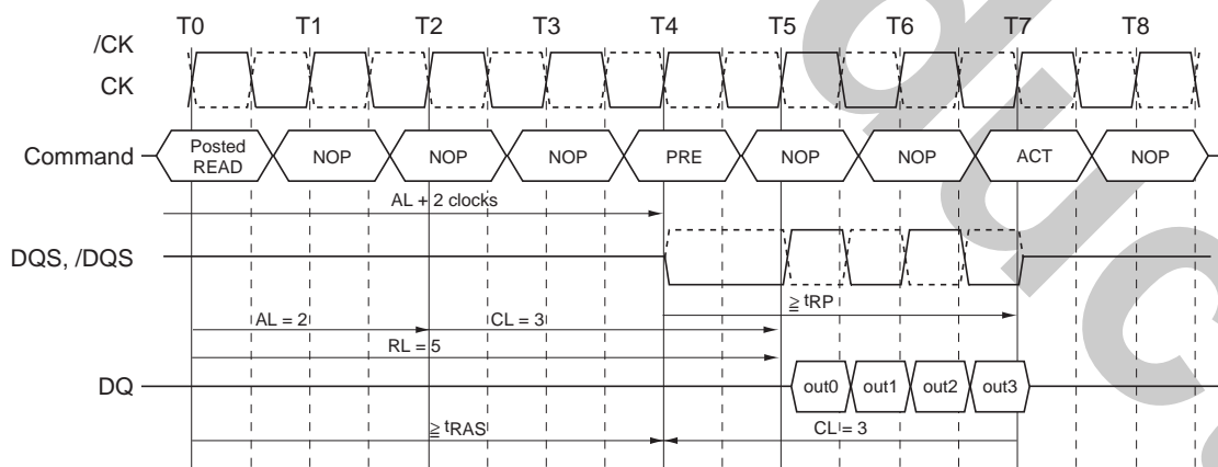
Burst Read Operation Followed by Precharge (RL = 5 (AL=2, CL=3))
