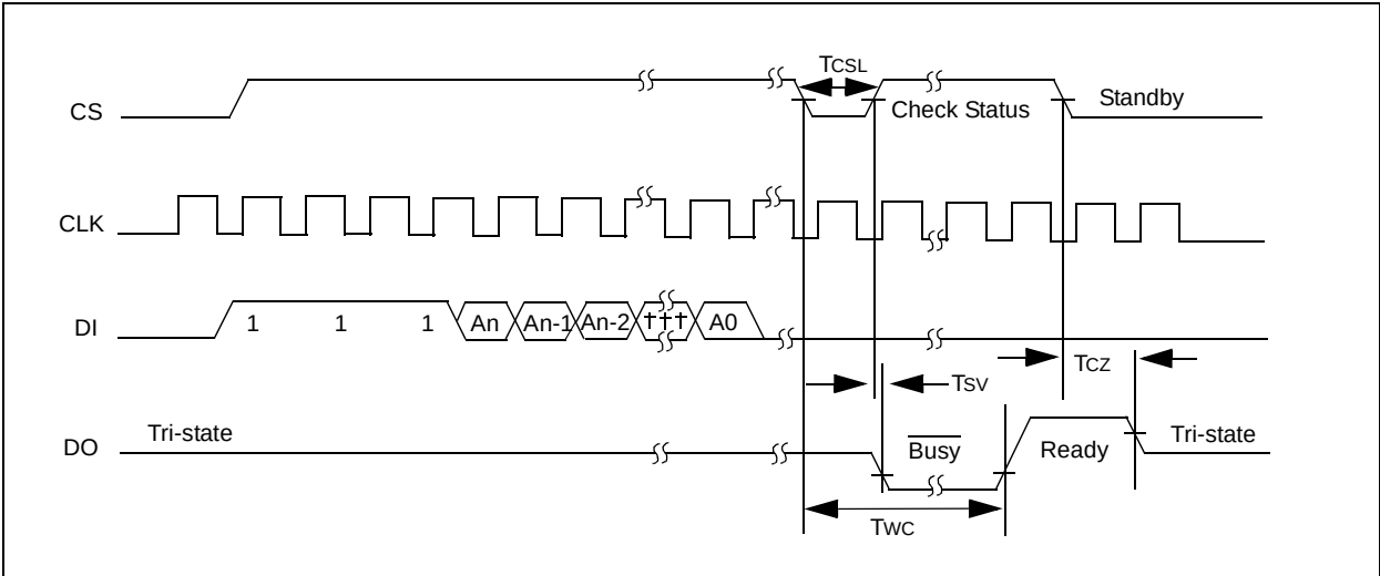
FIGURE 2-7: ERASE TIMING
