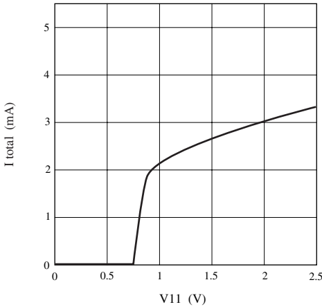
12. V_{CC} - I_{total}
