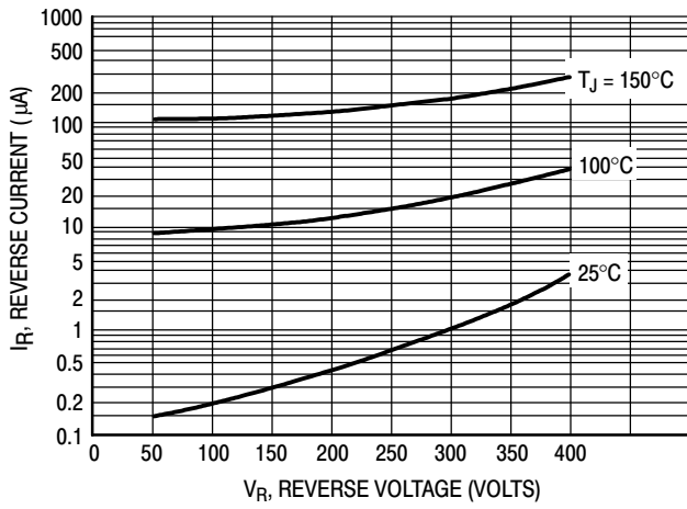
Figure 3. Typical Reverse Current, Per Leg
