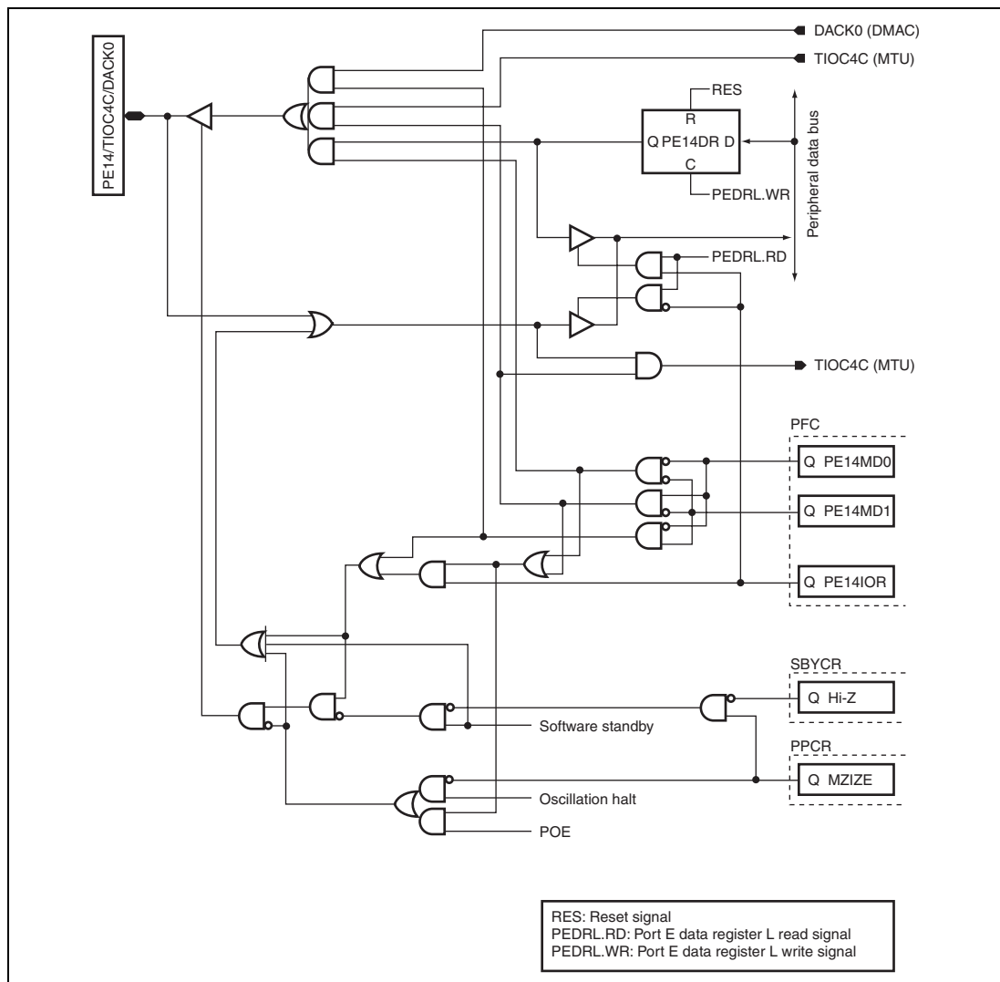
Figure D.41 PE14/TIOC4C/DACK0
