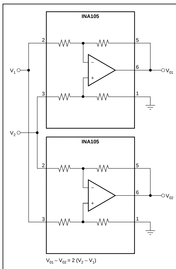
FIGURE 22. Differential Output Difference Amplifier.
