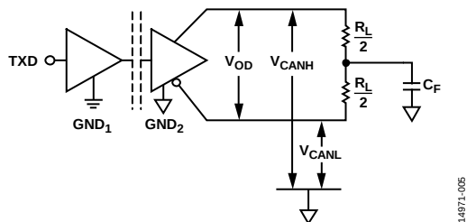
Figure 20. Driver Voltage Measurement
