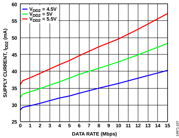
Figure 9. Supply Current ( I_{DD2} ) vs. Data Rate
