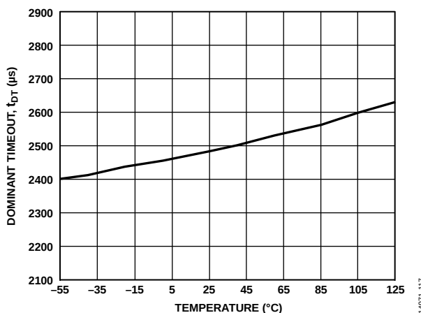
Figure 19. Dominant Timeout ( t_{\text{DT}} ) vs. Temperature
