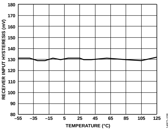
Figure 10. Receiver Input Hysteresis vs. Temperature
