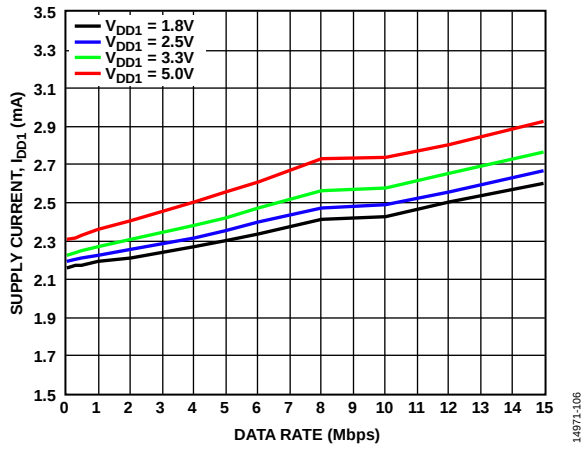
Figure 8. Supply Current ( I_{DD1} ) vs. Data Rate
