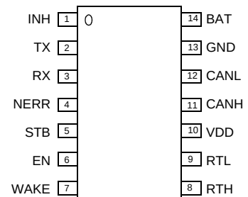
PIN CONNECTIONS
