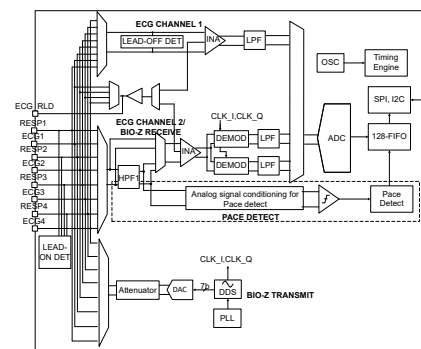
Figure 3-1. Block Diagram
