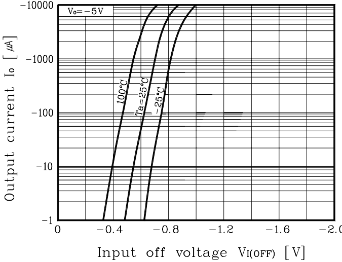
Fig. 2 I_O - V_{I(OFF)}
