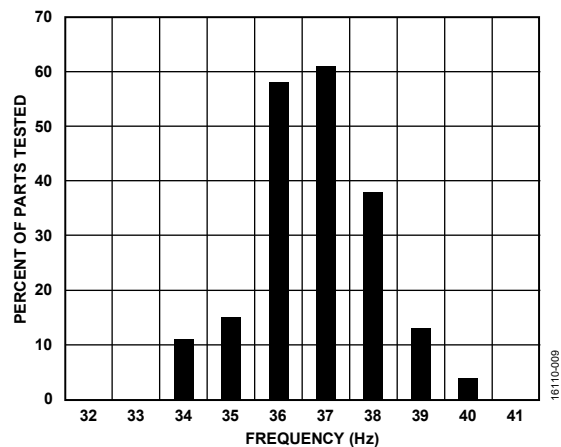
Figure 9. 32 kHz Clock Frequency Distribution (Default Settings, Before User Calibration: Register 0x4B = 0x2612)
