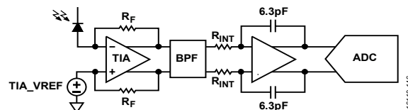
Figure 48. Receive Path Block Diagram
