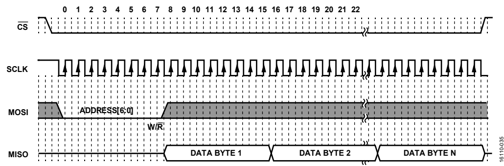
Figure 35. SPI Slave Read Clocking (Burst Read Mode, N Bytes)
