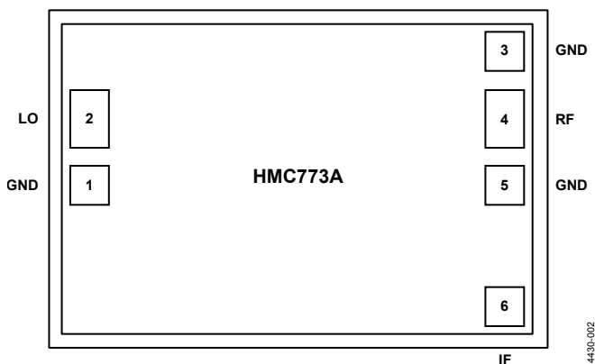
Figure 2. Pin Configuration
