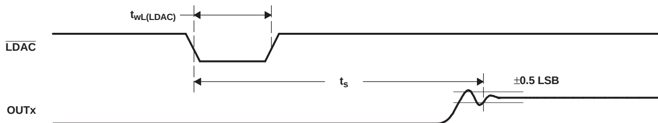
Figure 2. Output Timing
