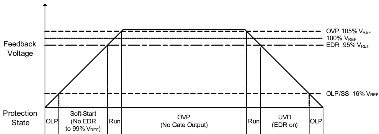
Figure 23. Soft Start and Protection States
