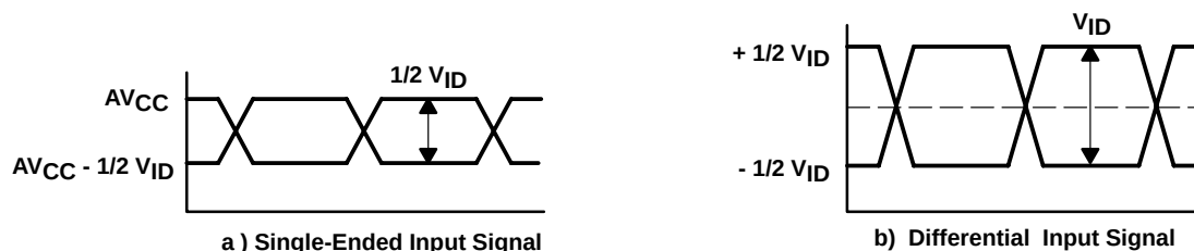
Figure 15. T.M.D.S. Inputs
