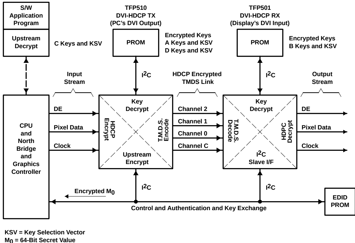
Figure 13. TI's HDCP Implementation for PC and Display System
