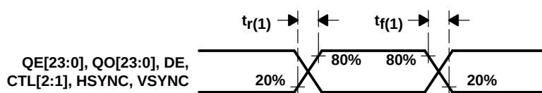
Figure 2. Rise and Fall Time of Data and Control Signals
