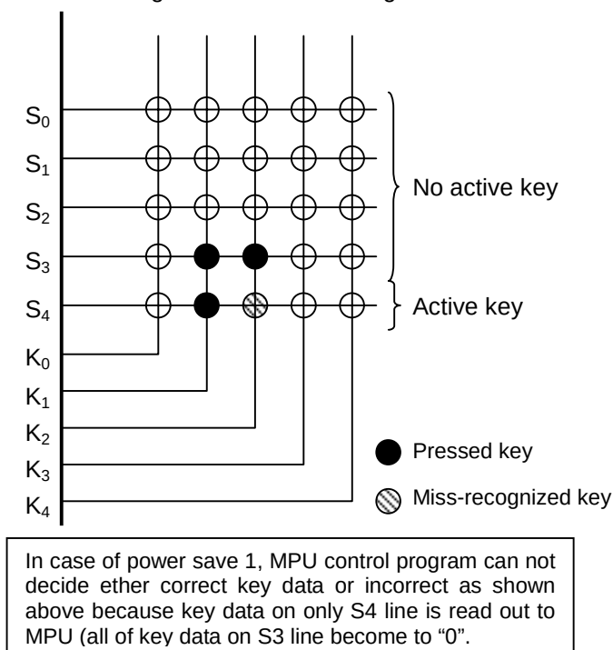
Fig. 2 Miss-recognition in power save 1
