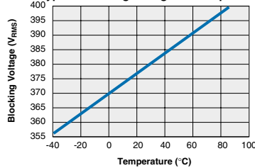
LBA110L - FormA Typical Blocking Voltage vs. Temperature
