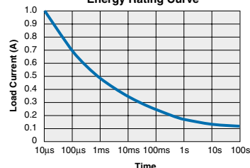
LBA110L Energy Rating Curve
