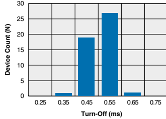
LBA110L - FormB Typical Turn-Off Time (N=50 Ambient Temperature = 25°C) (Load Current = 120mADC; I_F = 5\text{mADC} )
