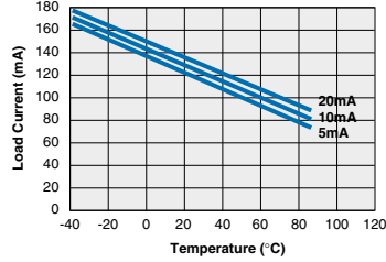
LBA110L - Form A Typical Load Current vs. Temperature
