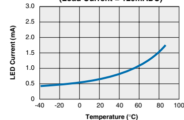
LBA110L - FormB Typical I_F for Switch Dropout vs. Temperature (Load Current = 120mADC)
