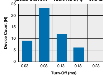
LBA110L - FormA Typical Turn-Off Time (N=50 Ambient Temperature = 25°C) (Load Current = 120mADC; I F = 5mADC)
