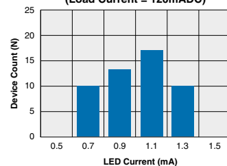
LBA110L - FormB Typical I F for Switch Dropout (N=50 Ambient Temperature = 25°C) (Load Current = 120mADC)
