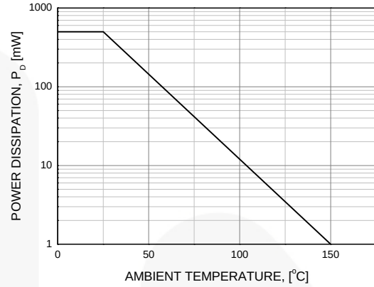
Figure 8. Power Deration
