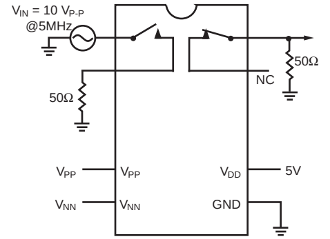
Crosstalk
