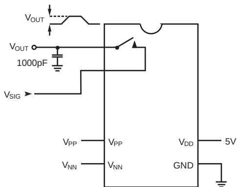
Charge Injection
