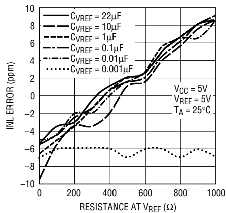
Figure 26. INL Error vs R_{VREF} (Large C)
