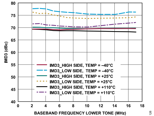
Figure 35. Transmitter Third-Order Intermodulation Distortion (IMD3) vs. Baseband Frequency, Transmitter Attenuation Code = 0, F1 = Baseband Frequency, F2 = Baseband Frequency + 1 MHz
