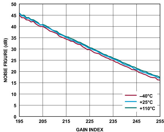
Figure 256. Receiver Noise Figure vs. Gain Index, Baseband Frequency = 2.1 kHz, ADC = Low Power
