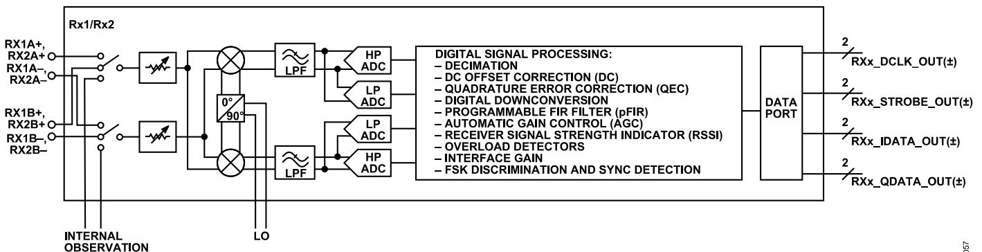
Figure 299. Receiver Architecture
