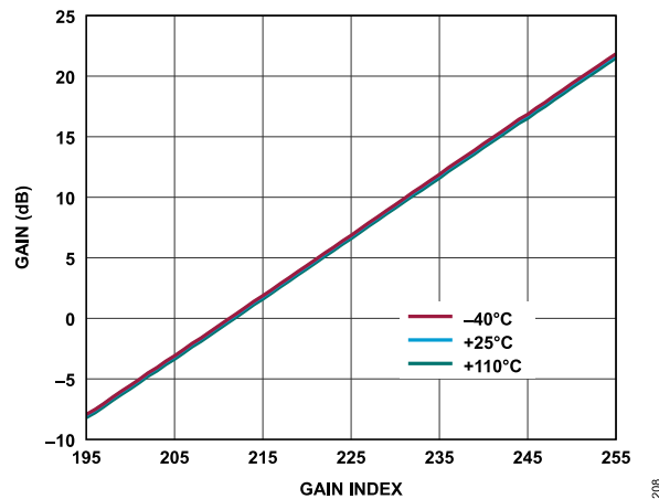
Figure 91. Receiver Absolute Gain (Complex) vs. Gain Index, Baseband Frequency = 5.6 MHz, ADC = High Performance, P_{OUT} = -9.6 dBFS
