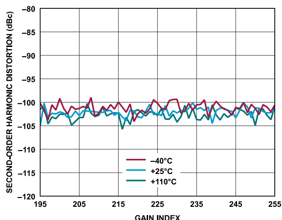
Figure 181. Receiver Second-Order Harmonic Distortion vs. Gain Index, Baseband Frequency = 2.1 kHz, ADC = High Performance
