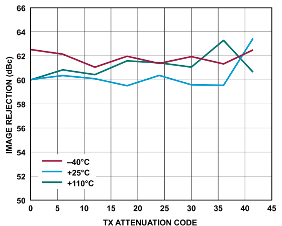
Figure 111. Transmitter Image Rejection vs. Transmitter Attenuation Code, Baseband Frequency = 18 MHz, Backoff = 0.2 dBFS, Initialization Calibration Only
