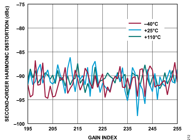
Figure 96. Receiver Second-Order Harmonic Distortion vs. Gain Index, Baseband Frequency = 5.6 MHz, ADC = Low Power
