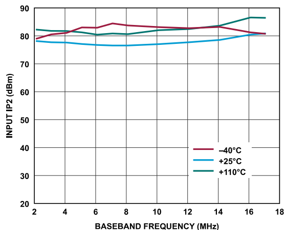
Figure 51. Receiver Input IP2 vs. Baseband Frequency, ADC = High Performance, F1 = Baseband Frequency, F2 = Baseband Frequency + 1 MHz, Gain Index = 255
