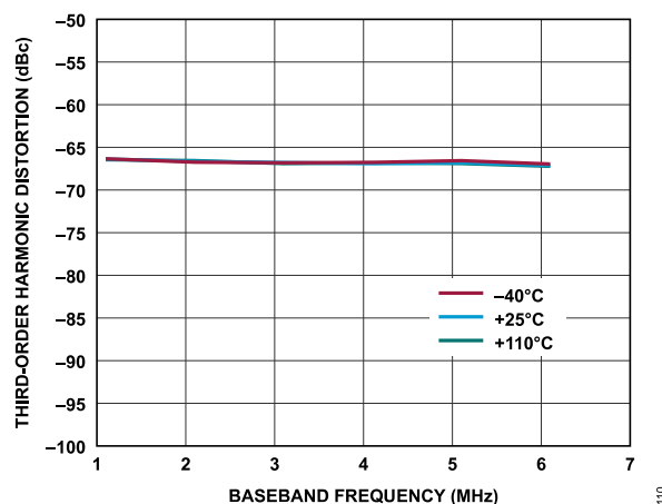
Figure 17. Receiver Third-Order Harmonic Distortion vs. Baseband Frequency, Gain Index = 255, ADC = High Performance
