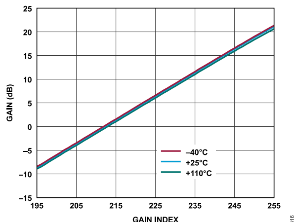
Figure 178. Receiver Absolute Gain (Complex) vs. Gain Index, Baseband Frequency = 2.1 kHz, ADC = High Performance, P_{OUT} = -9.6 dBFS
