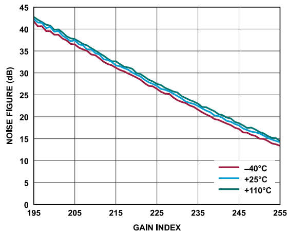
Figure 255. Receiver Noise Figure vs. Gain Index, Baseband Frequency = 2.1 kHz, ADC = High Performance
