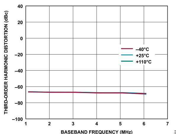
Figure 19. Receiver Third-Order Harmonic Distortion vs. Baseband Frequency, Gain Index = 255, ADC = Low Power
