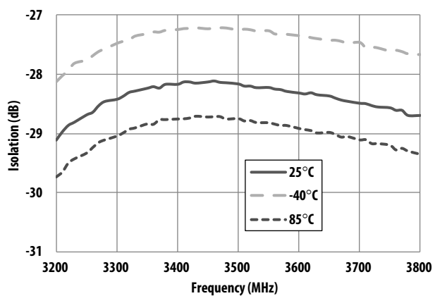
Figure 38. Isolation vs Frequency and Temperature
