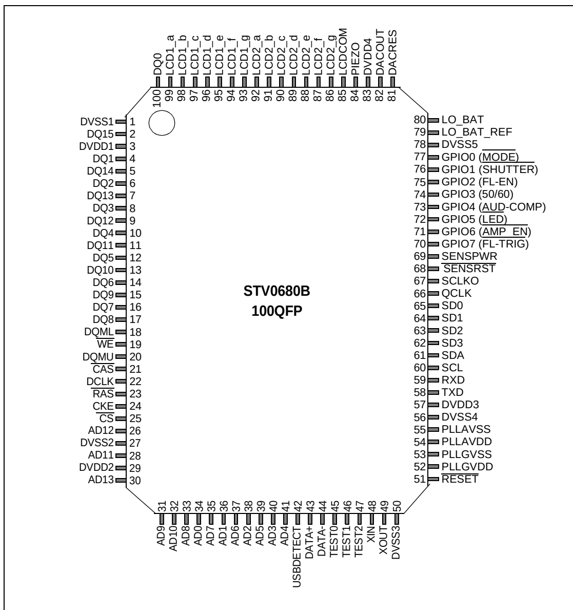
Figure 11 : STV0680B pinout in 100QFP package
