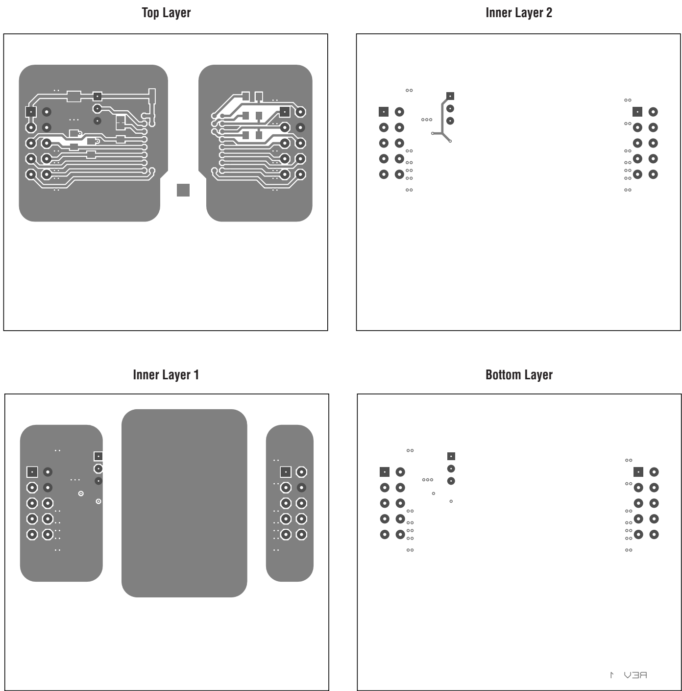
Figure 14b. LTM2883 Low EMI Demo Board Layout (DC1748A)
