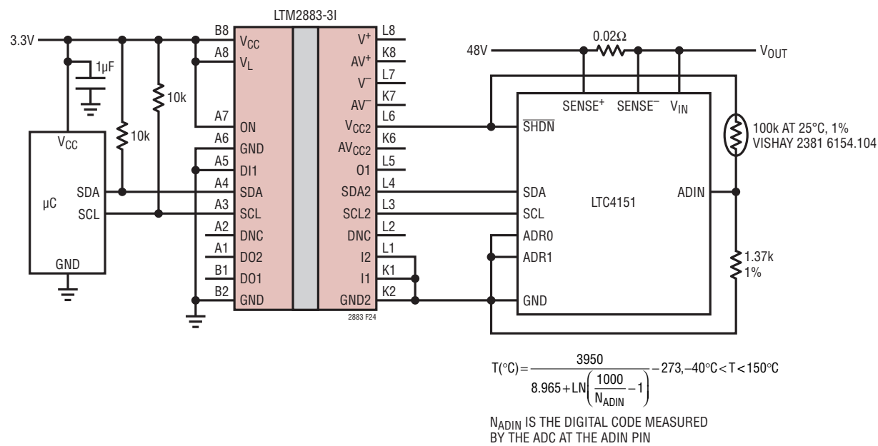
Figure 24. Isolated I²C Voltage, Current and Temperature Power Supply Monitor
