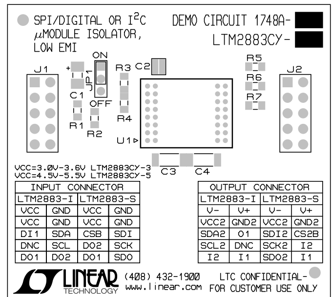
Figure 14a. LTM2883 Low EMI Demo Board Layout
