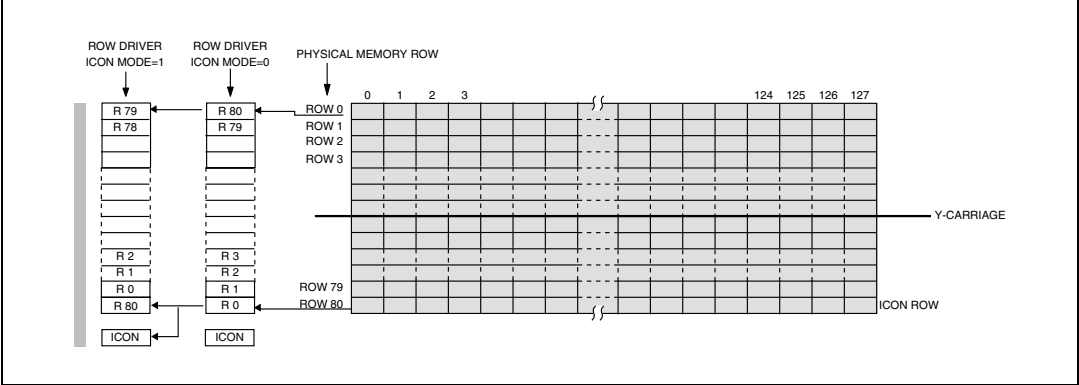
Figure 21. Memory Rows vs. Row drivers mapping with MY=1, MUX81, icon mode 0,1 scroll pointer=0
