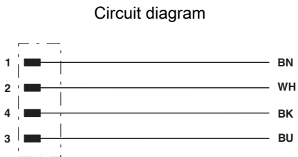
M12 x 1 socket, angled
