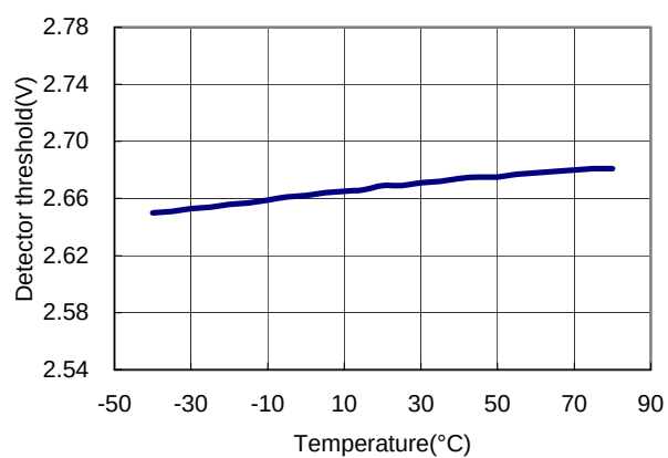
Detector threshold=2.7V
