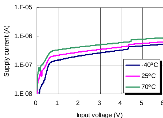
Detector threshold=4.4V
