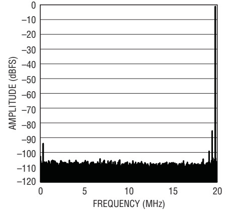
LTC2141-12: 64k Point FFT, f_{IN} = 140\text{MHz} , -1\text{dBFS} , 40\text{Msps}
