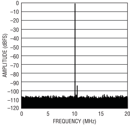
LTC2141-12: 64k Point FFT, f_{IN} = 30\text{MHz} , -1\text{dBFS} , 40\text{Msps}
