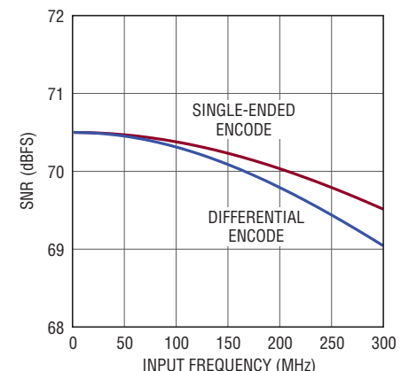
LTC2141-12: SNR vs Input Frequency, -1\text{dBFS} , 40\text{Msps} , 2\text{V} Range
