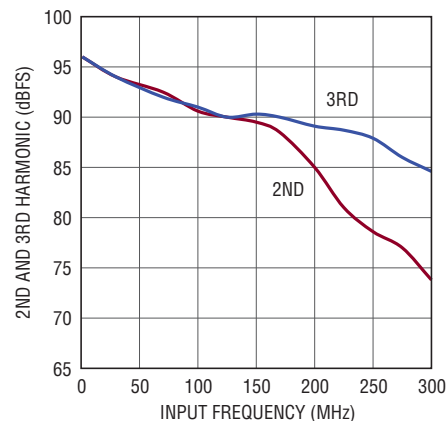
LTC2141-12: 2nd, 3rd Harmonic vs Input Frequency, -1\text{dBFS} , 40\text{Msps} , 1\text{V} Range
