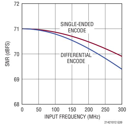
LTC2140-12: SNR vs Input Frequency, -1\text{dBFS} , 25\text{Mps} , 2\text{V} Range
