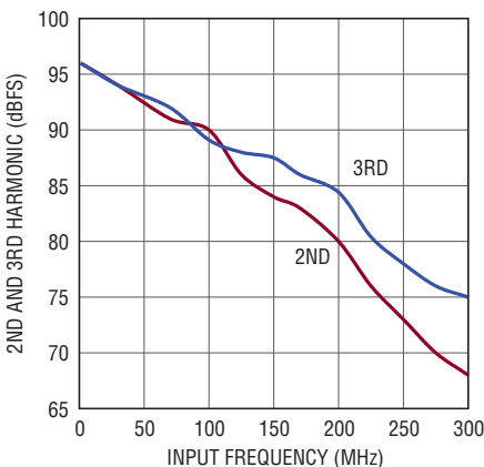
LTC2141-12: 2nd, 3rd Harmonic vs Input Frequency, -1\text{dBFS} , 40\text{Msps} , 2\text{V} Range
