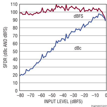
LTC2142-12: SFDR vs Input Level, f_{IN} = 70\text{MHz} , 65Msps, 2V Range
