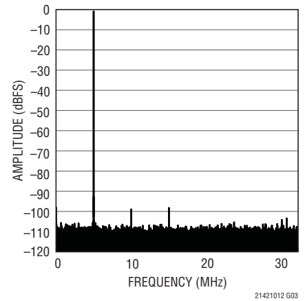
LTC2142-12: 64k Point FFT, f_{IN} = 5\text{MHz} , -1\text{dBFS} , 65Msps
