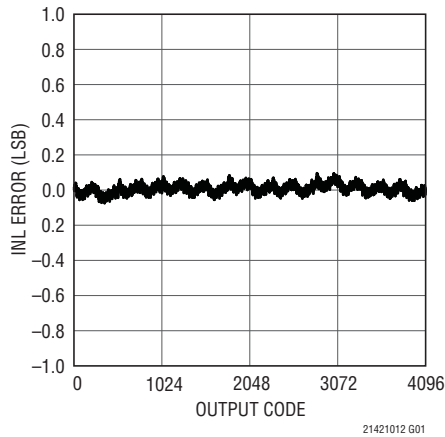
LTC2142-12: Integral Non-Linearity (INL)
