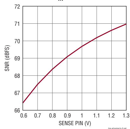
LTC2142-12: SNR vs SENSE, f_{IN} = 5\text{MHz} , -1dBFS
