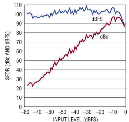
LTC2141-12: SFDR vs Input Level, f_{IN} = 70\text{MHz} , 40\text{Msps} , 2\text{V} Range
