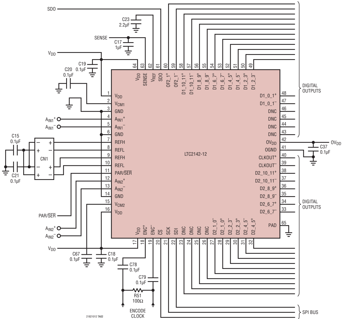
LTC2142 Schematic
