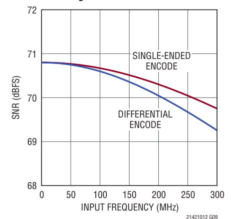
LTC2142-12: SNR vs Input Frequency, -1\text{dBFS} , 65Msps, 2V Range
