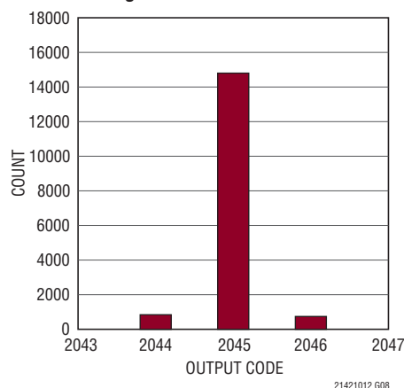
LTC2142-12: Shorted Input Histogram
