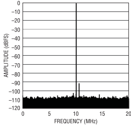
LTC2141-12: 64k Point FFT, f_{IN} = 70\text{MHz} , -1\text{dBFS} , 40\text{Msps}
