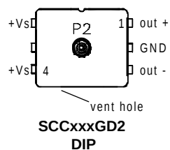
SCC.. Button Sensor
