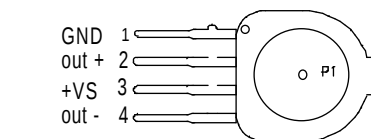
SCC.. Button Sensor
