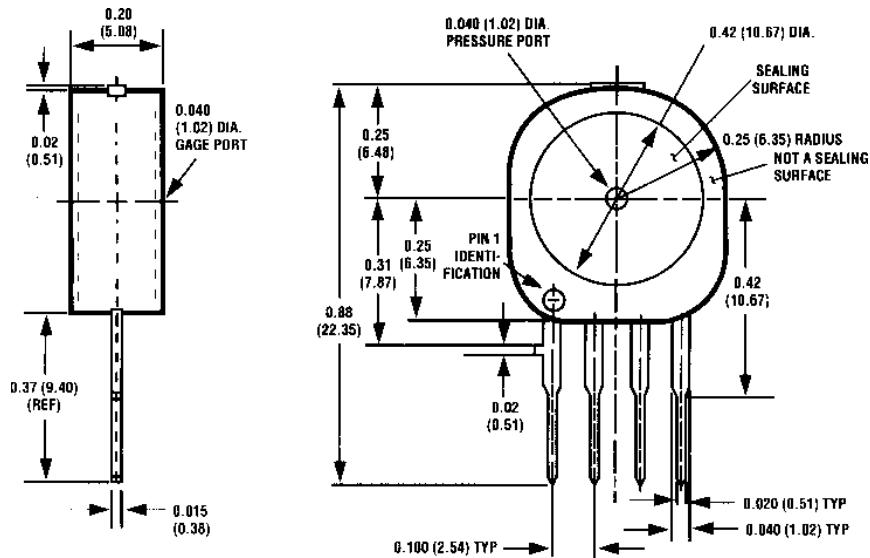
Button Package
