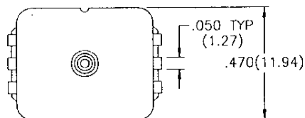
Basic Sensor DIP "D2" Package
