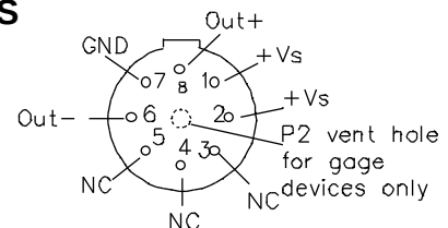
TO Can (bottom view)
