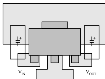
Figure 1. SOT-89 Board Layout
