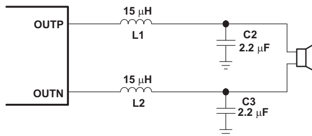
Figure 38. Typical LC Output Filter, Cutoff Frequency of 27 kHz, Speaker Impedance = 4 Ω
