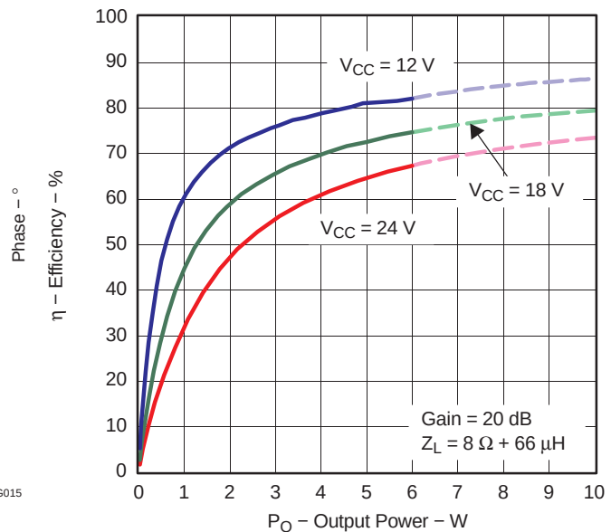
EFFICIENCY vs OUTPUT POWER (BTL)
