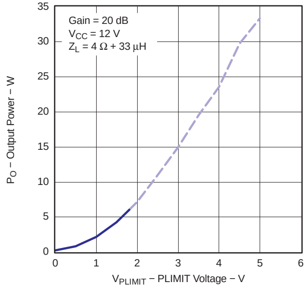
OUTPUT POWER vs PLIMIT VOLTAGE (BTL)
