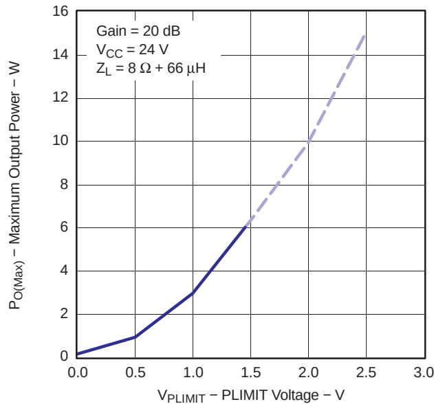
MAXIMUM OUTPUT POWER vs PLIMIT VOLTAGE (BTL)
