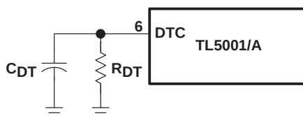
Figure 2. Soft-Start Circuit
